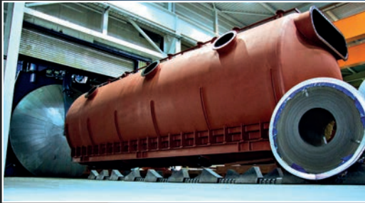
Workshop rubber linings: The best possible rubber lining quality is achieved in Steuler autoclaves at high temperatures and pressures.
